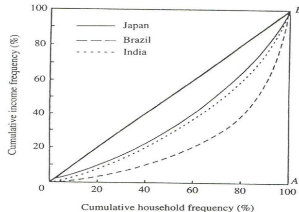
FIG. 7.1 Lorenz curves for Japan, Brazil, and India
